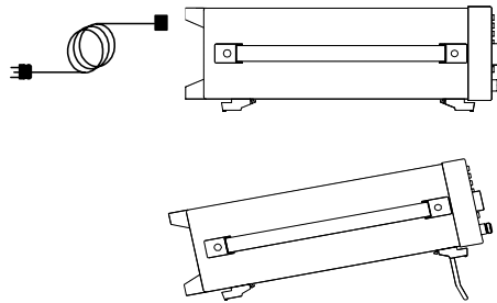
Figure 2-1 Plug in and angle adjustment
