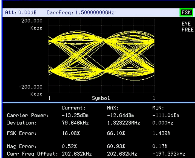
Figure 3-28 FSK Eye Diagram
