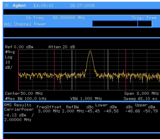
Figure 4-6 Adjacent Channel Power Measurement
