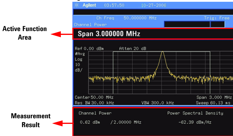
Figure 4-4 Channel Power Measurement
