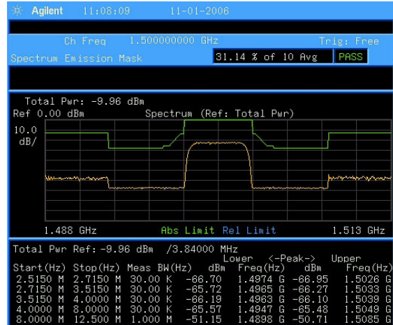
Figure 4-8 Spectrum Emission Mask
