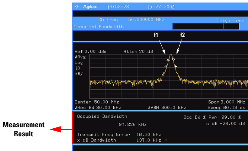
Figure 4-5 Occupied Bandwidth Measurement
