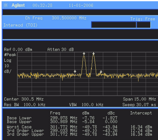
Figure 4-7 TOI Measurement
