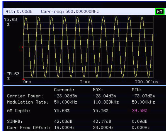
Figure 3-26 AM demodulation analysis
