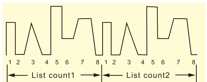
List Sequence
