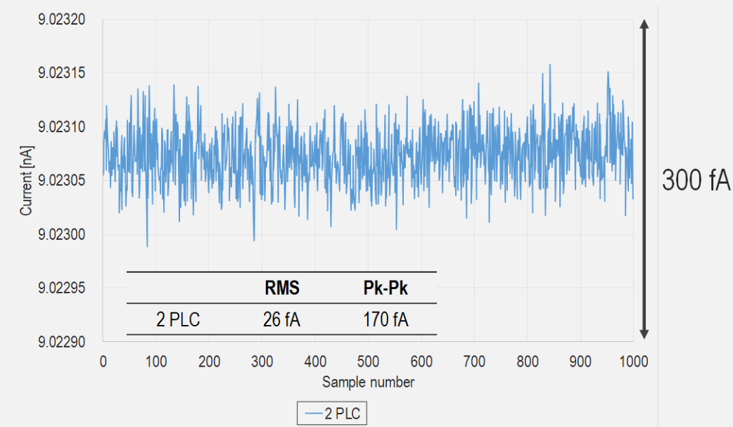
Figure 11. Measurement noise, 10 nA range, 1 GΩ load, 9 V, triax cable (3 m)
