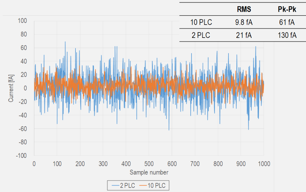
Figure 10. Measurement noise, 10 nA range, no load, 0 V, triax cable (3 m)
