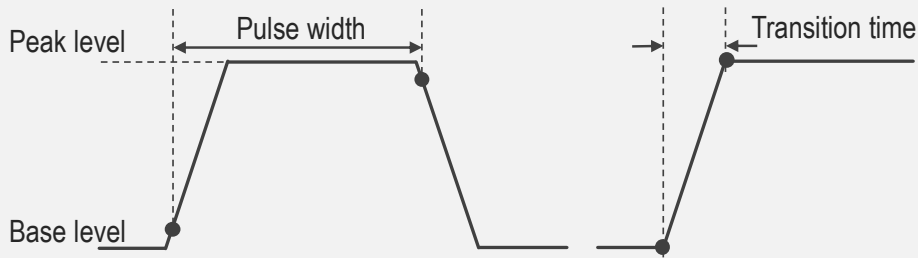
Figure 7. Definition of the pulse parameters and the transition time
