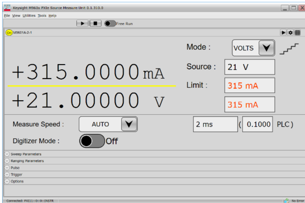
Figure 6. M9601A soft front panel
