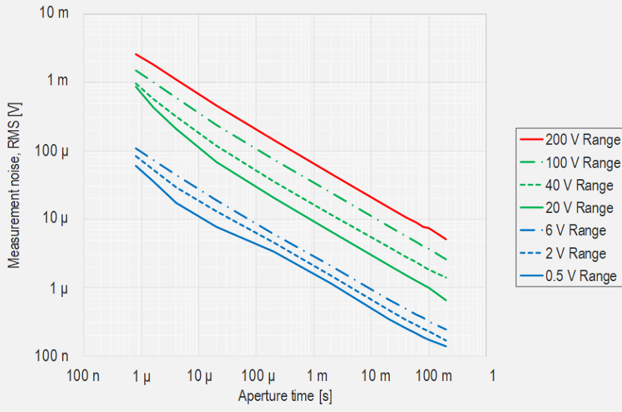
Figure 8. Voltage measurement noise vs. measurement aperture time
