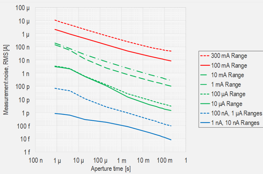
Figure 9. Current measurement noise vs. measurement aperture time
