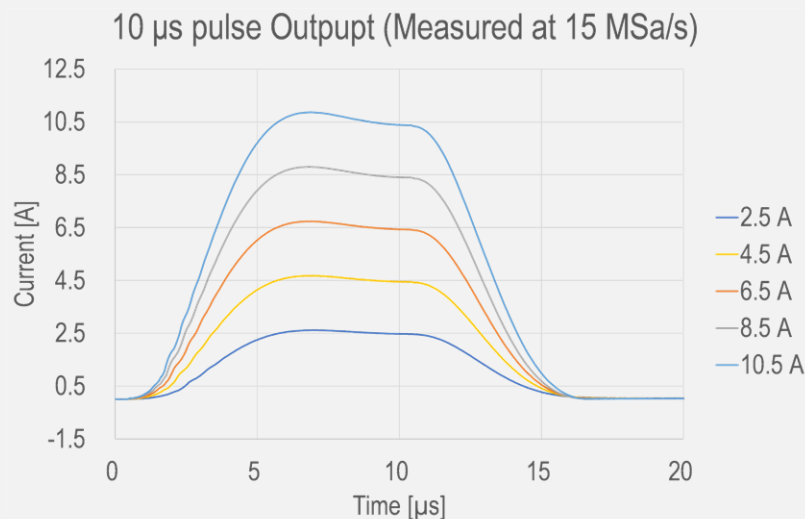
Figure 1. Narrow pulse output with measuring at 15 MSa/s sampling rate
