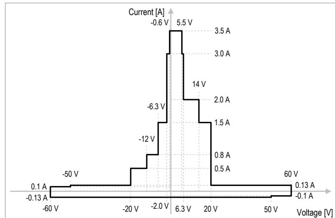
Figure 6. DC voltage and current output range (With mode for the chassis supporting 6 A backplane pin current capacity for 12 V rail.)
