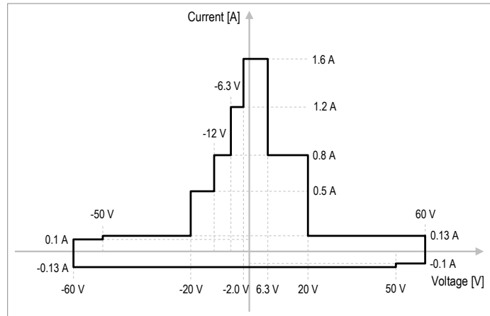
Figure 7. DC voltage and current output range (With mode for the chassis supporting 4 A backplane pin current capacity for 12 V rail.)
