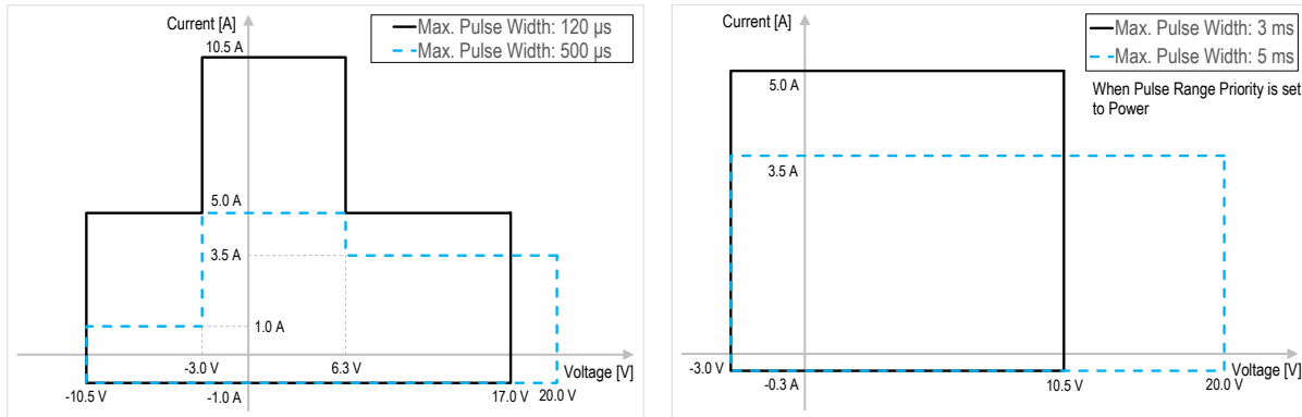
Figure 8. Pulsed voltage and current output range
